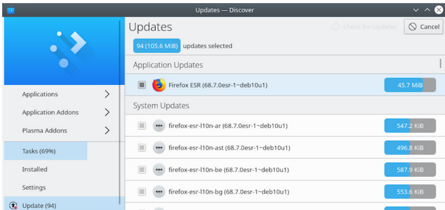
update progress
