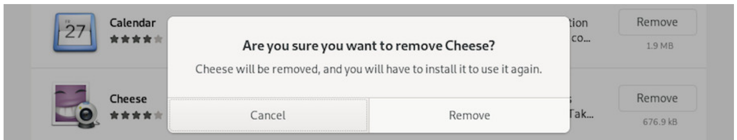
confirmation
