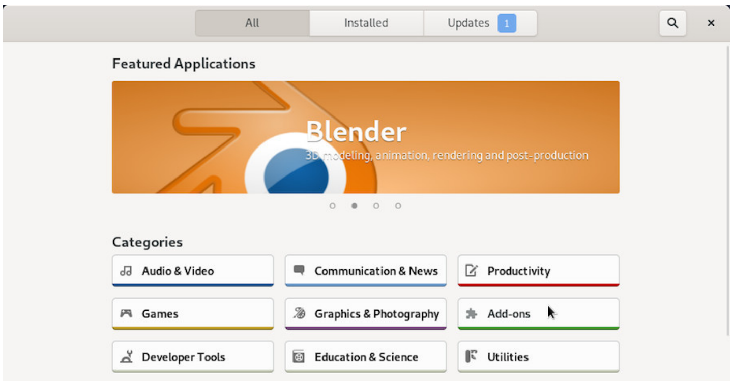
launching “Software”
